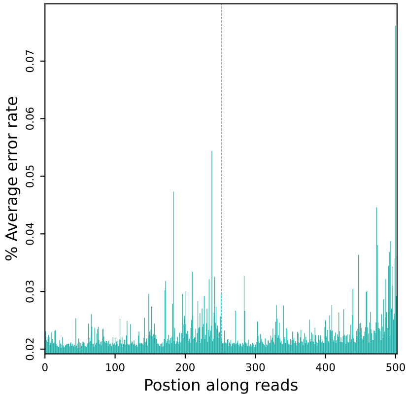
Error rate distribution along reads (R10520)
